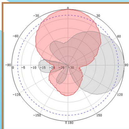
Radiation Pattern 868 MHz
